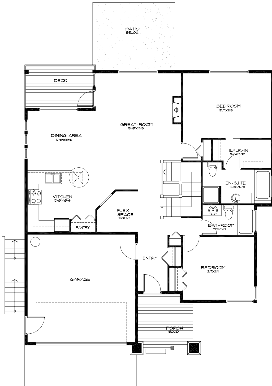
1 MAIN FLOOR PLAN Scale 1/4" = 1'-0" MAIN FLOOR 1360 SQ. FT GARAGE 385 SQ. FT
