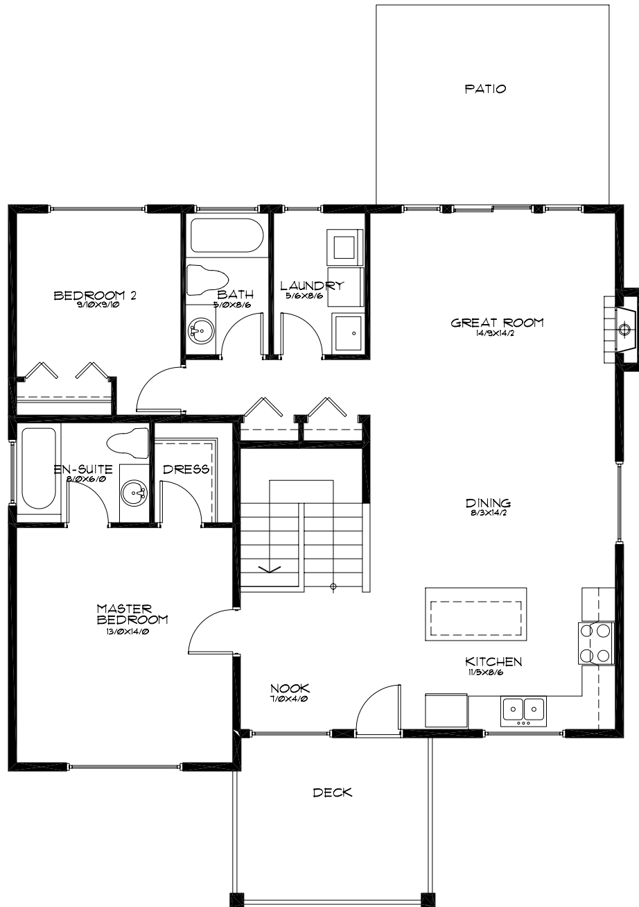
1 A2.2 UPPER FLOOR PLAN Scale 1/4" = 1'-0" MAIN FLOOR AREA 1212 SF.
