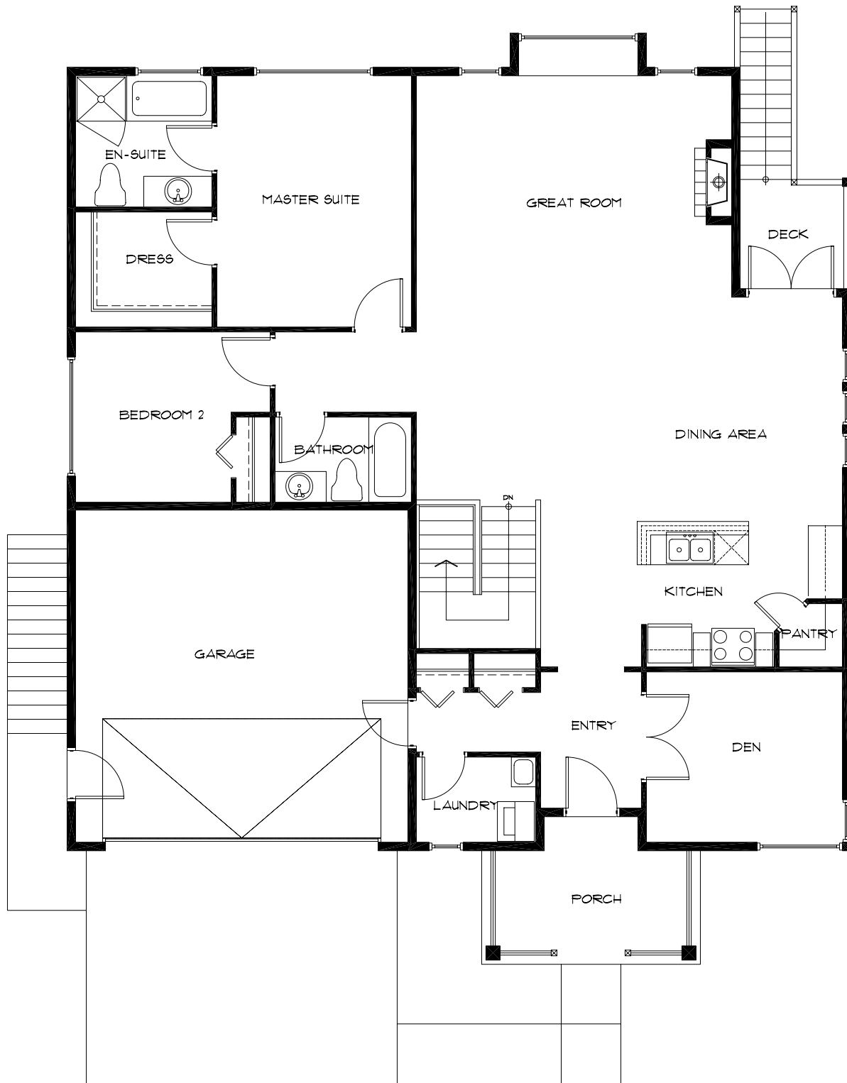
1 MAIN FLOOR PLAN A2.2 Scale 1/4" = 1'-0"
