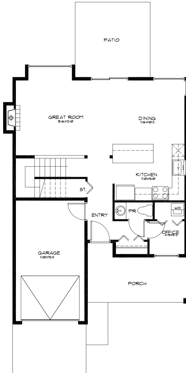
1 MAIN FLOOR PLAN A2.2 Scale 1/4" = 1'-0"
