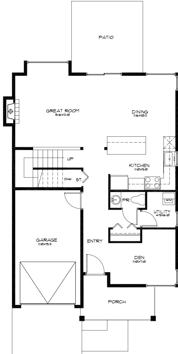
1 A2.2 MAIN FLOOR PLAN Scale 1/4" = 1'-0" MAIN FLOOR AREA 821 S.F. INC STAIR
